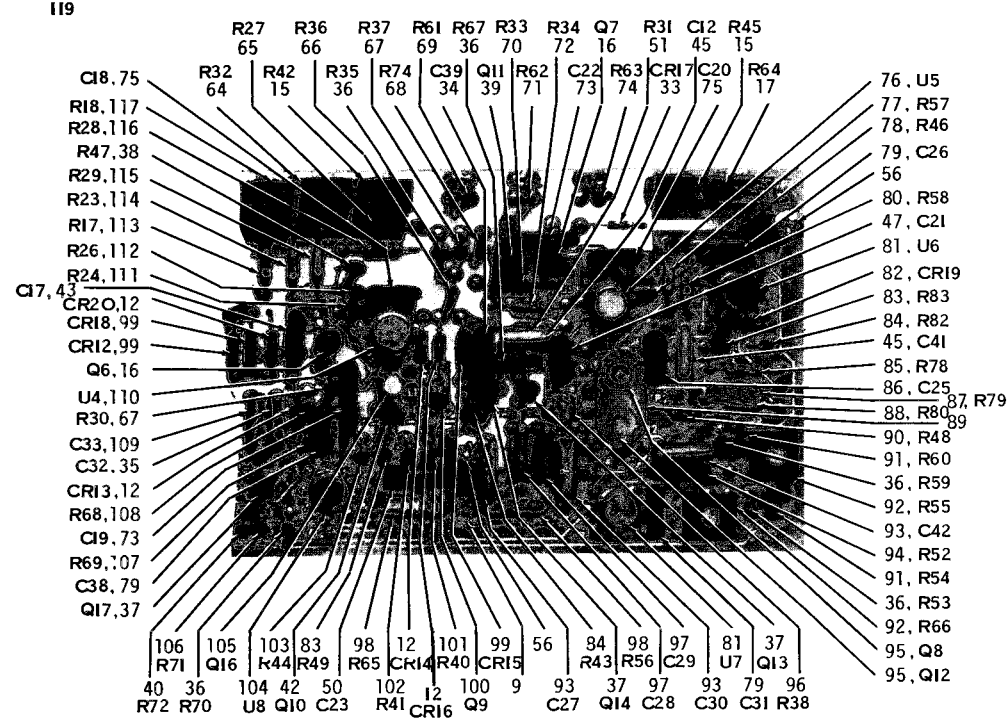
B-15. Ac converter assembly
