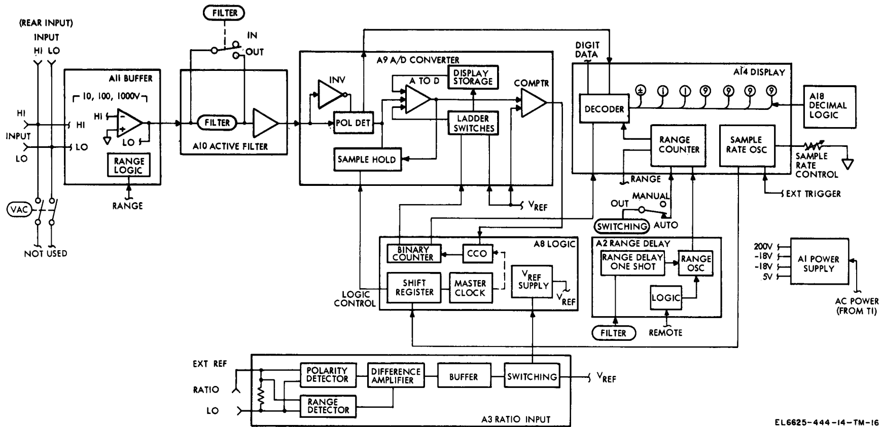
Figure 5-1. Voltmeter block diagram.
