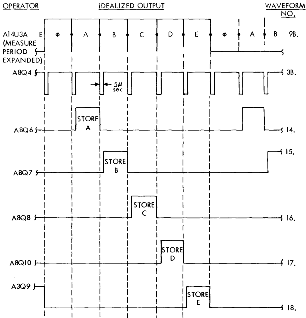
Figure 5-5 (3) Timing and synchrony diagram (sheet 3 of 3).
