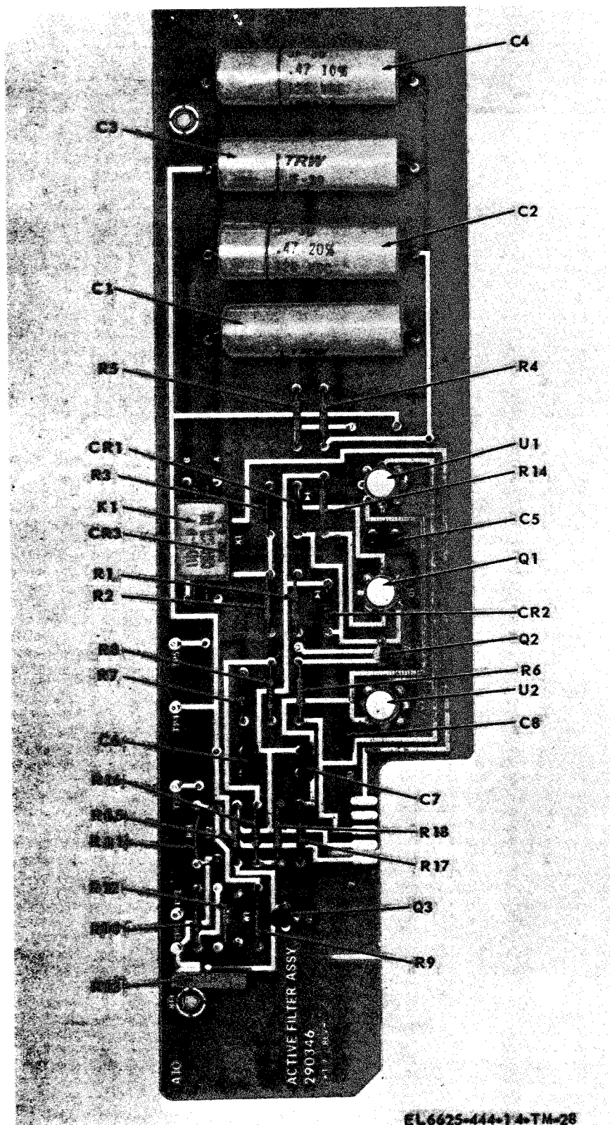
Figure 6-4. Active filter (A10) component parts.
