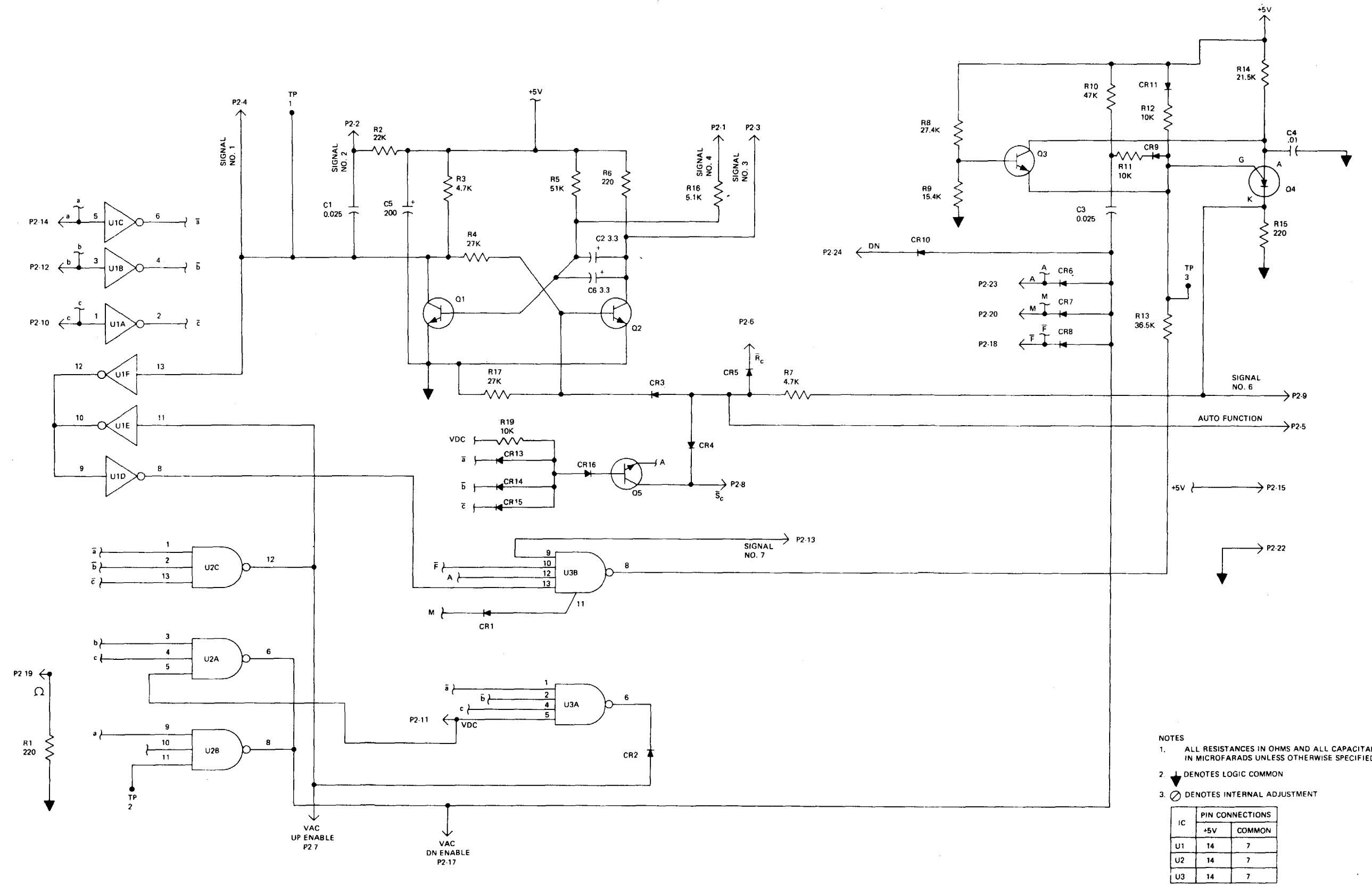
Figure FO-7. Range delay (A2) schematic diagram.
