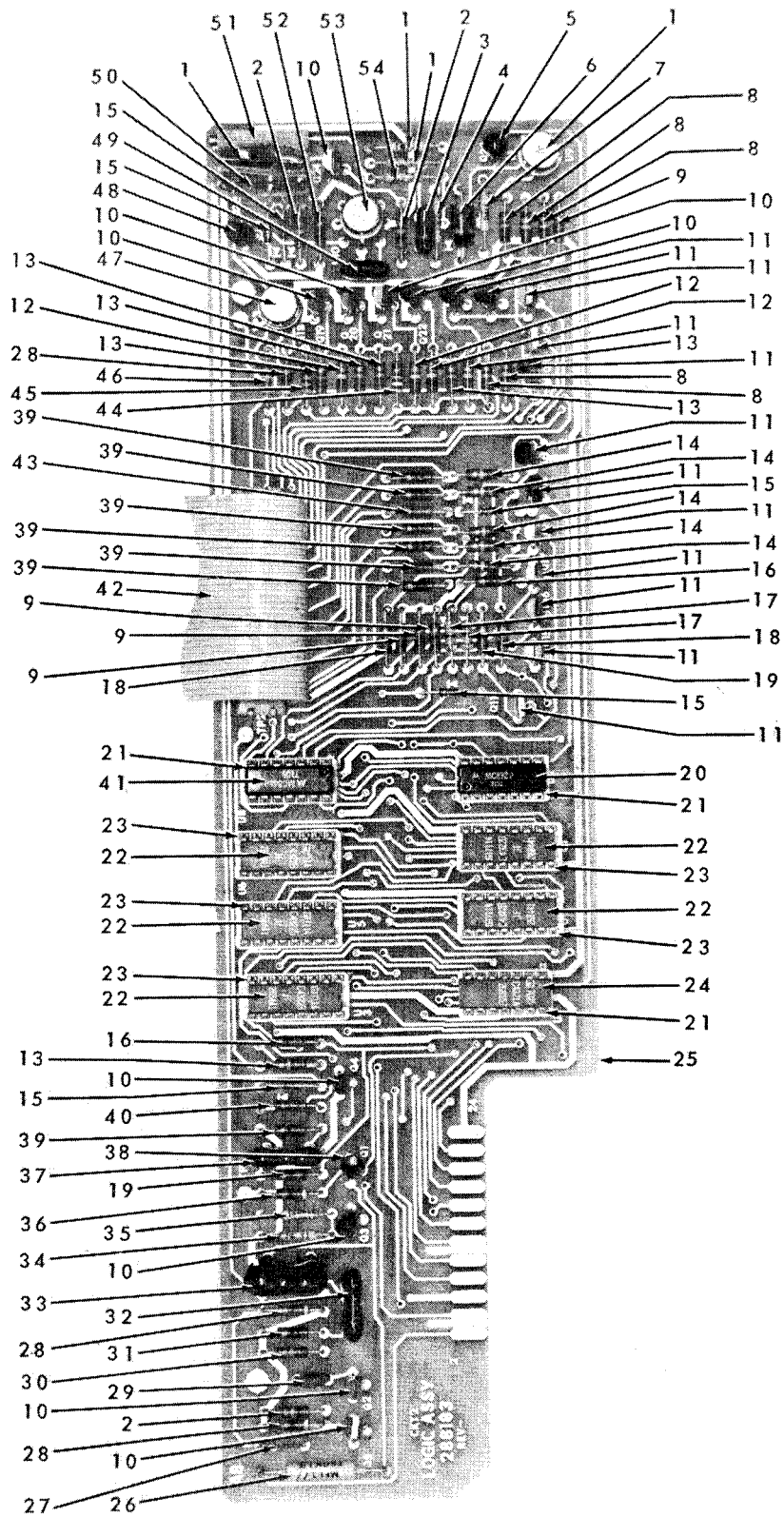
Figure 6. Logic assembly.
