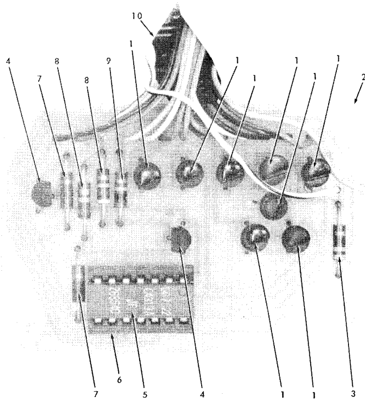
Figure 14. Decimal logic assembly.
