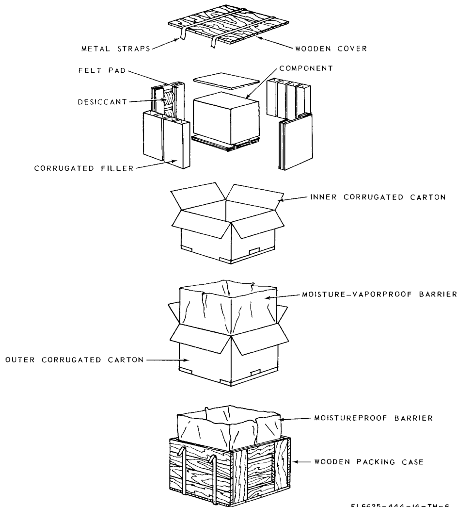
Figure 2-1. Packaging diagram
