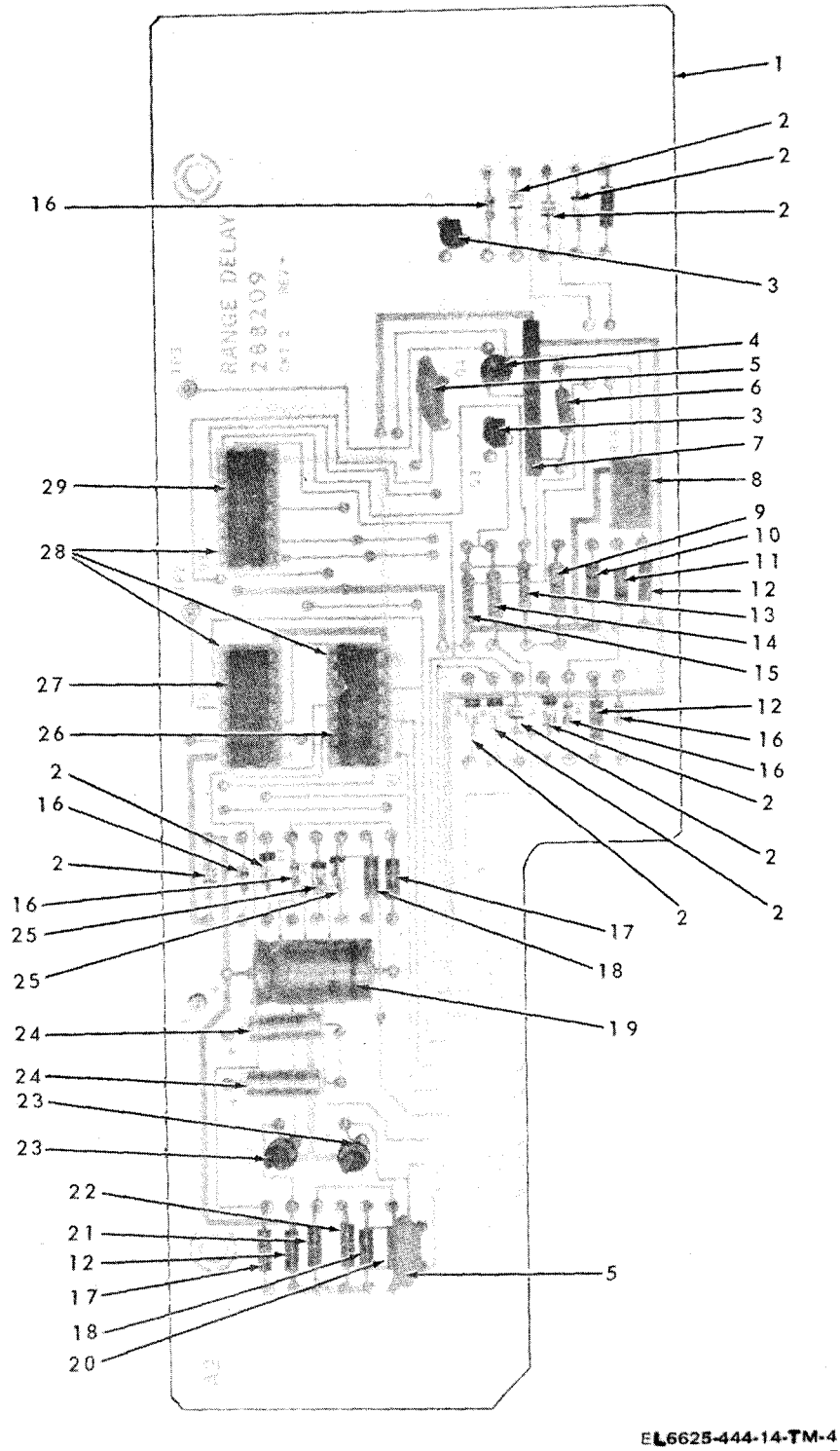
Figure 4. Range delay assembly
