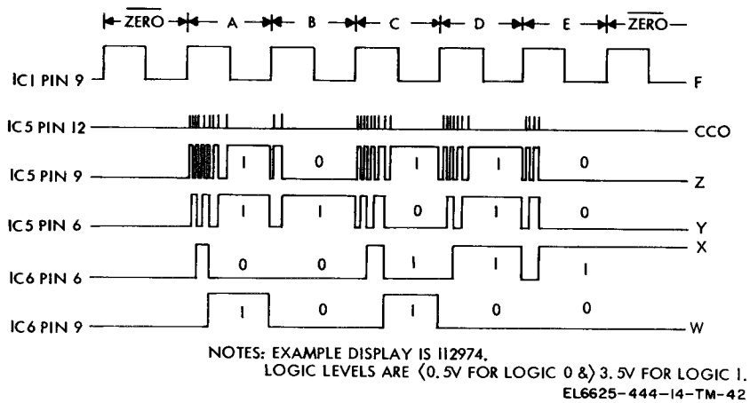
Figure 6-18. 16-State binary counter waveforms.
