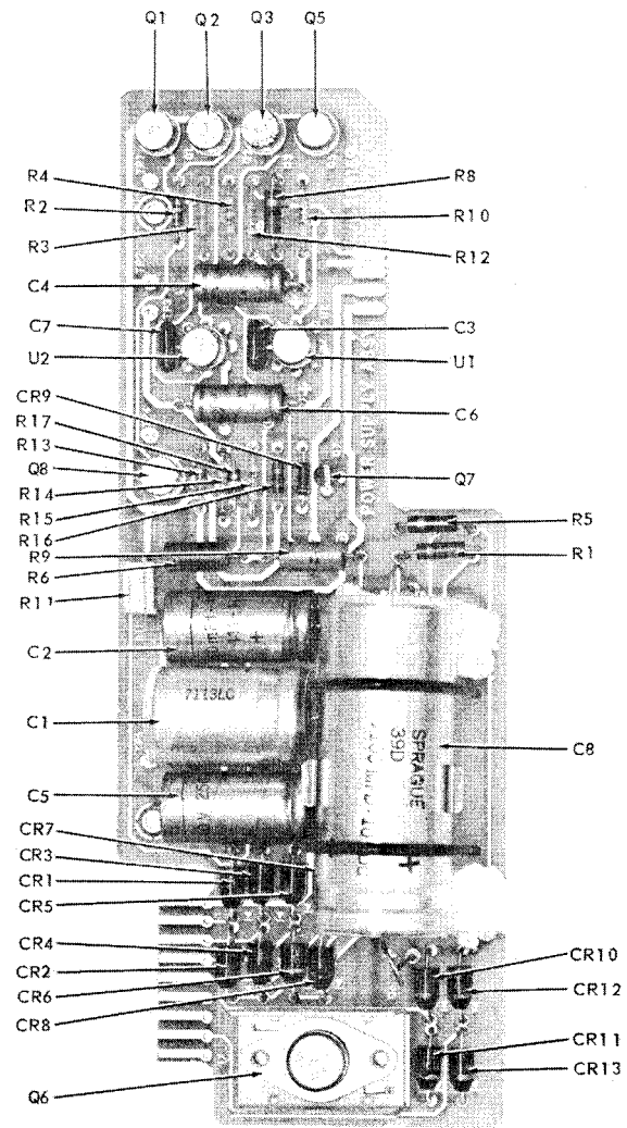
Figure 6-9. Power supply (A1) component parts.
