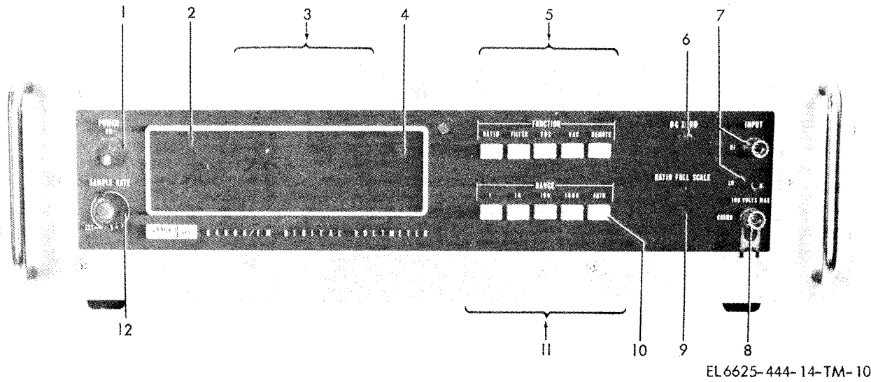
Figure 3-2 ①. Controls, connectors, and indicators (front panel).
