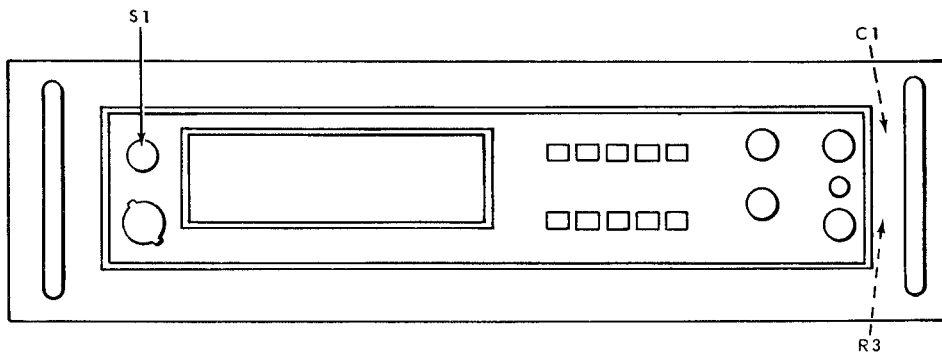
Figure 6-12. Front panel (A16) component parts.
