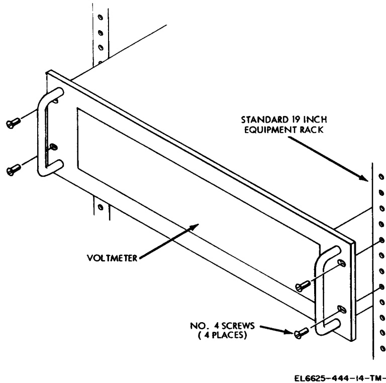
Figure 2-2. Rack installation.
