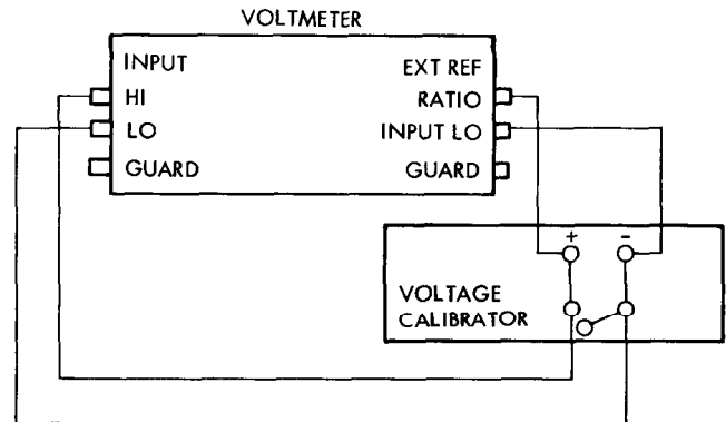
Figure 3-3. Operational check equipment connections
