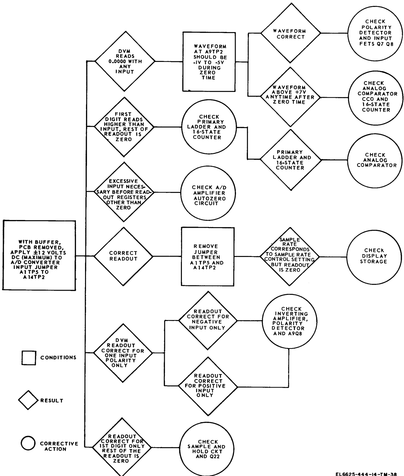
Figure 6-14. A-to-D converter and logic troubleshooting.
