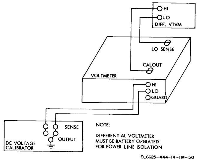
Figure 6-26. Alignment equipment connections.
