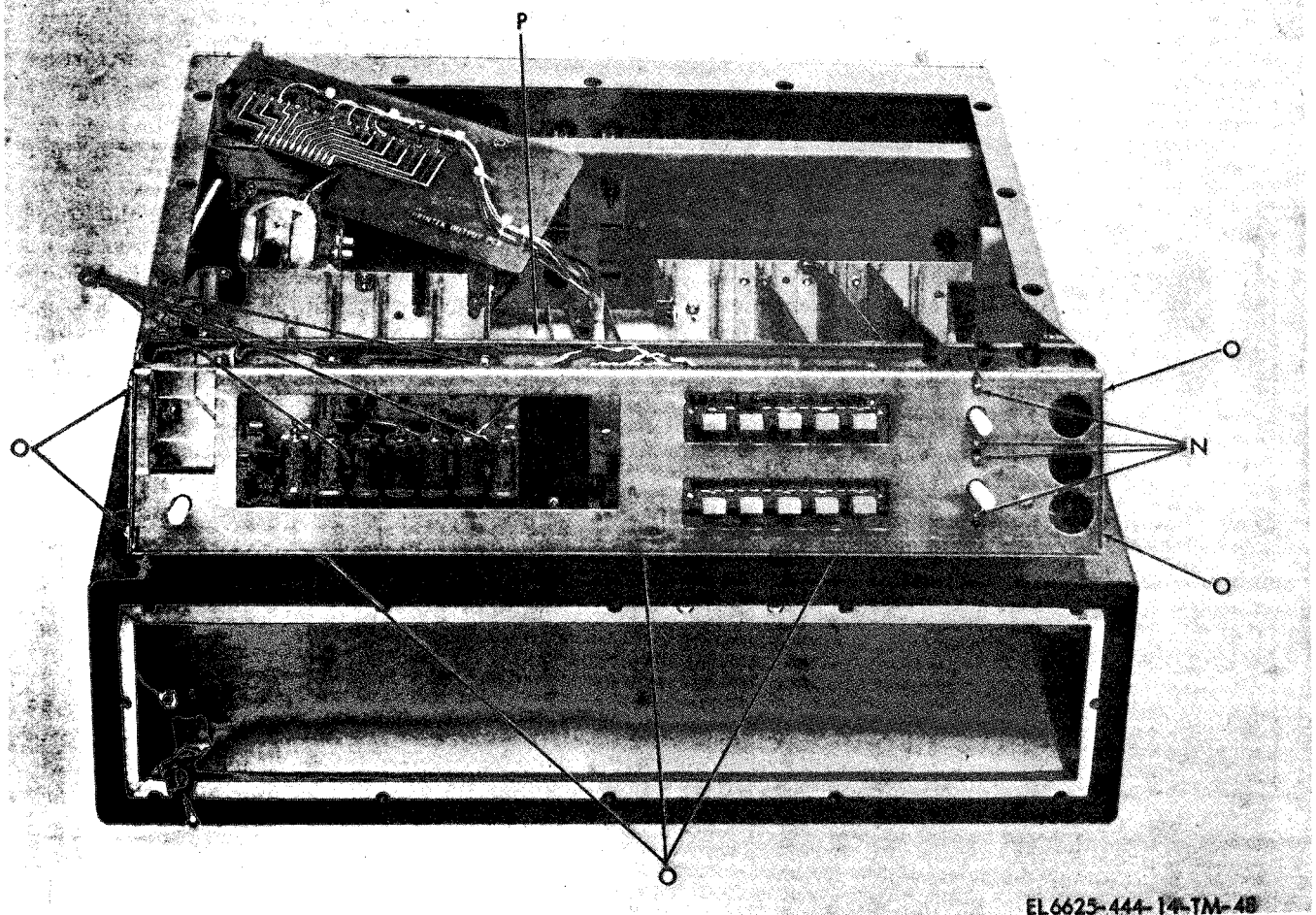
Figure 6-24. Disassembly sequence (n through u ).
