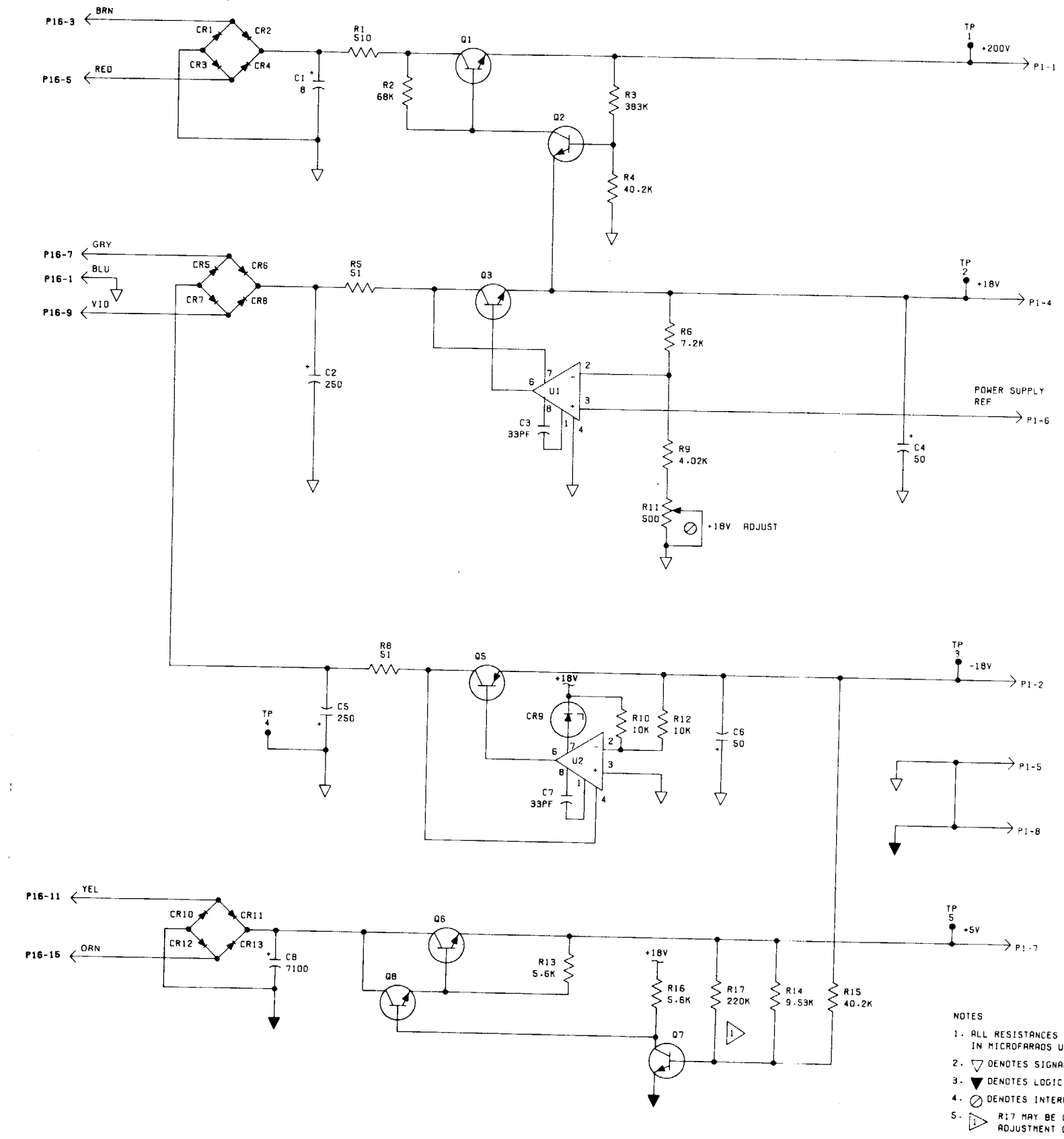
Figure FO-8. Power supply (A1) schematic diagram.
