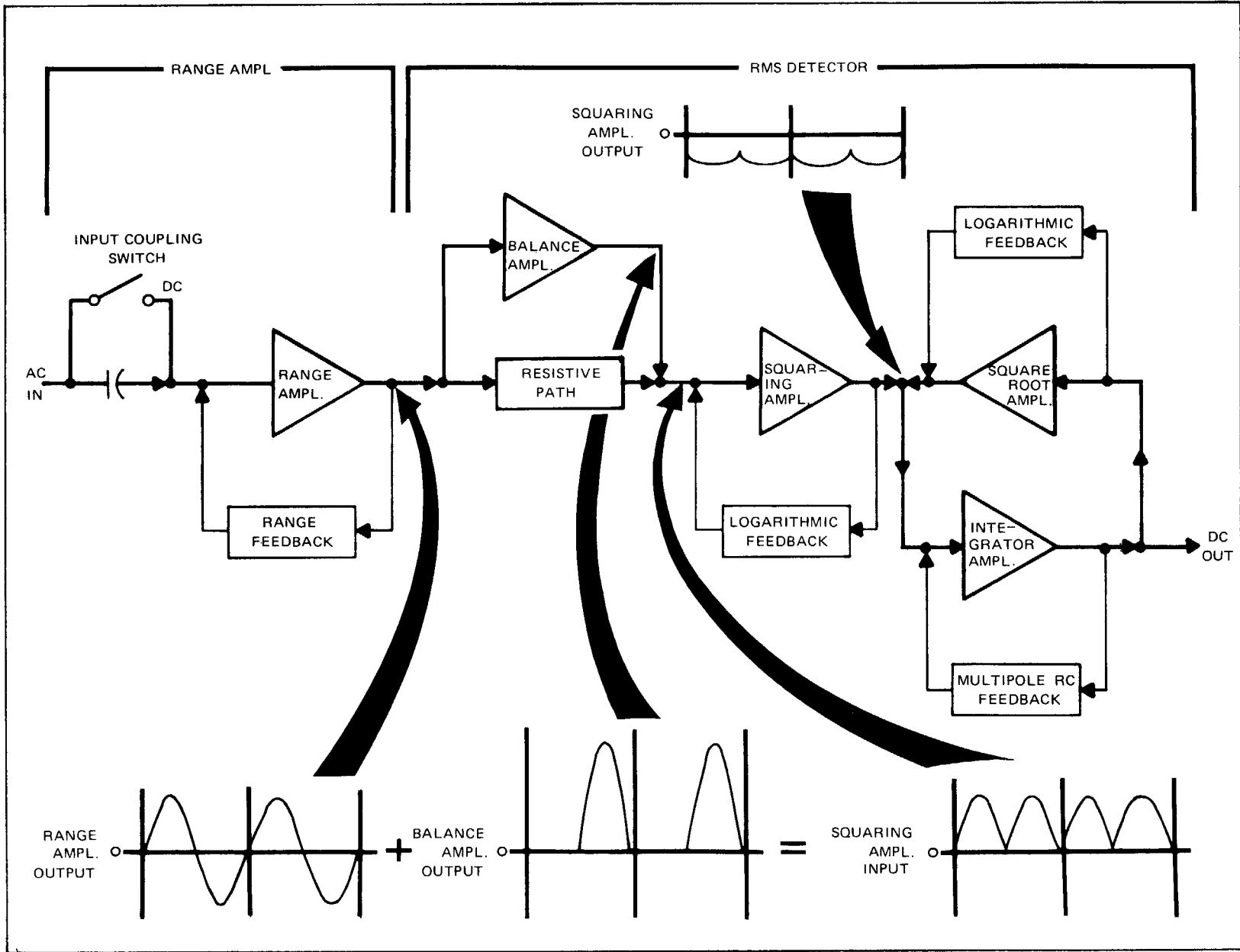
Figure 7-2. Ac converter, block diagram.
