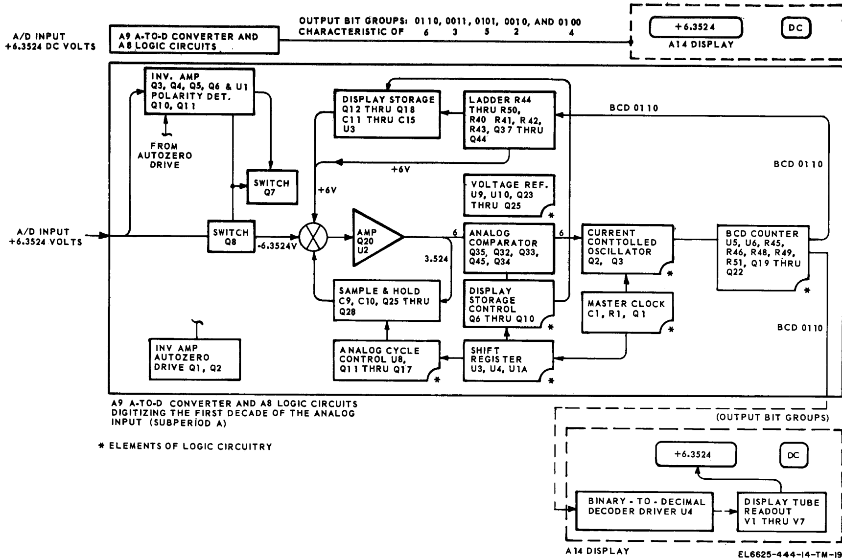
Figure 5-4. A/D converter block diagram.
