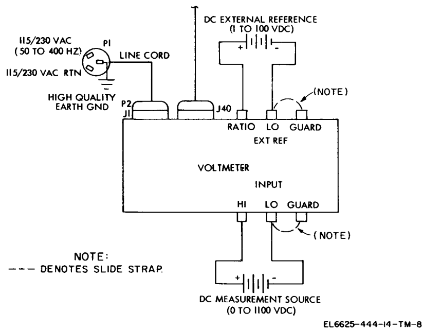
Figure 2-3. Equipment connections.
