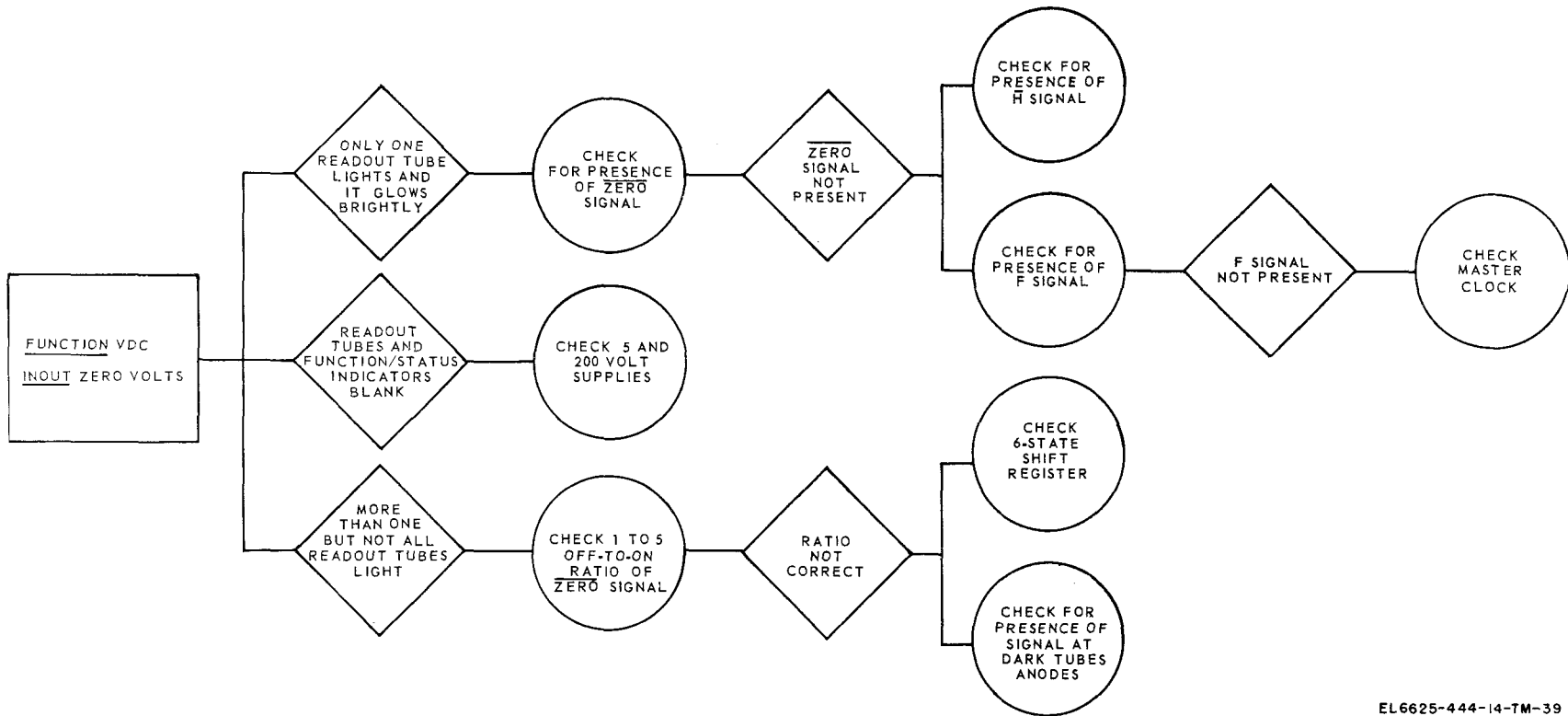
Figure 6-15. Display troubleshooting.
