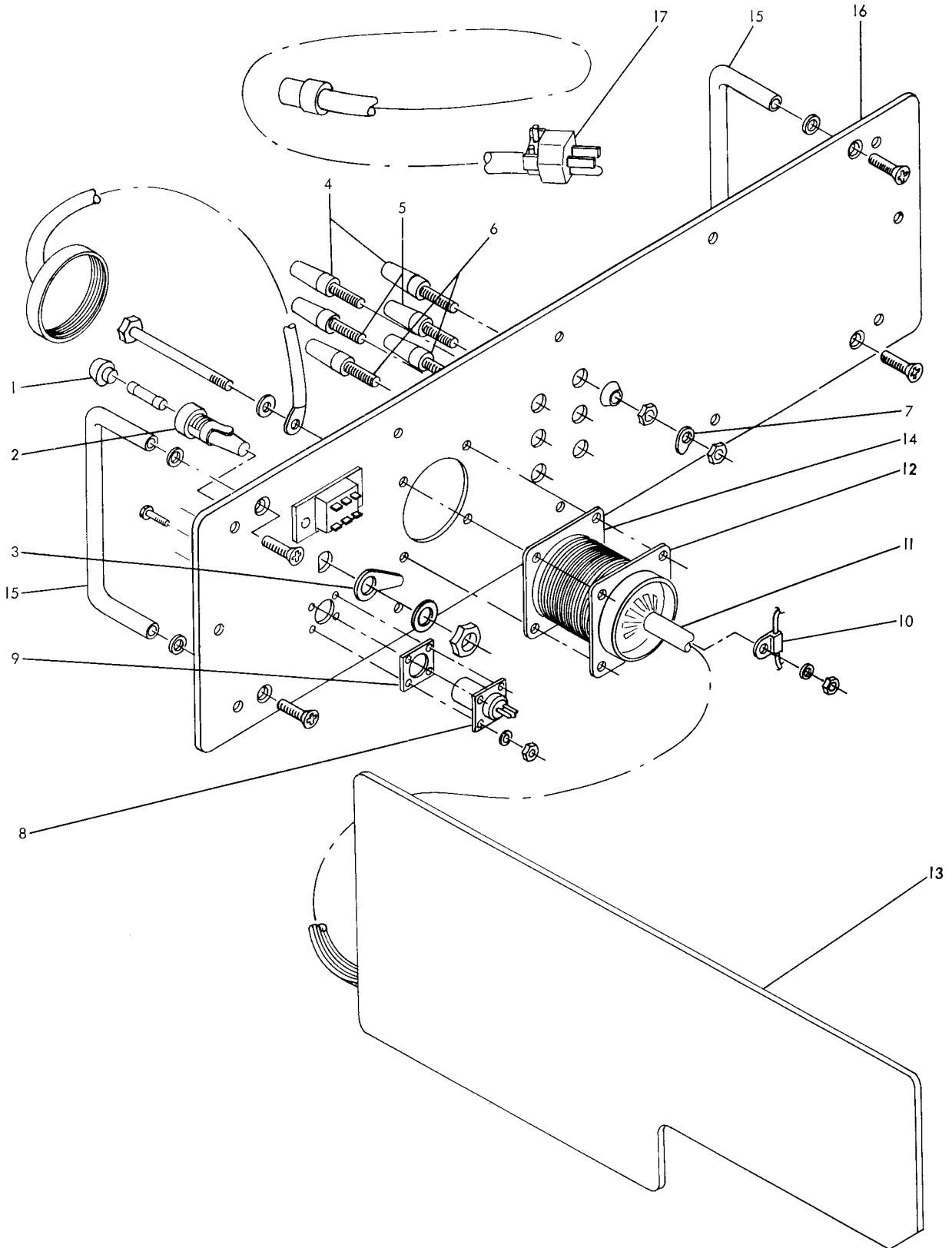
Figure 12. Rear assembly.
