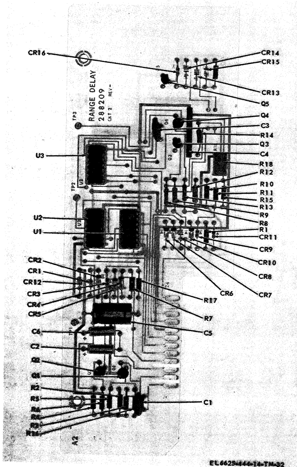
Figure 6-8. Range delay (A2 ) component parts.
