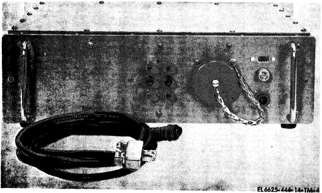
Figure 1-3. Rear panel.
