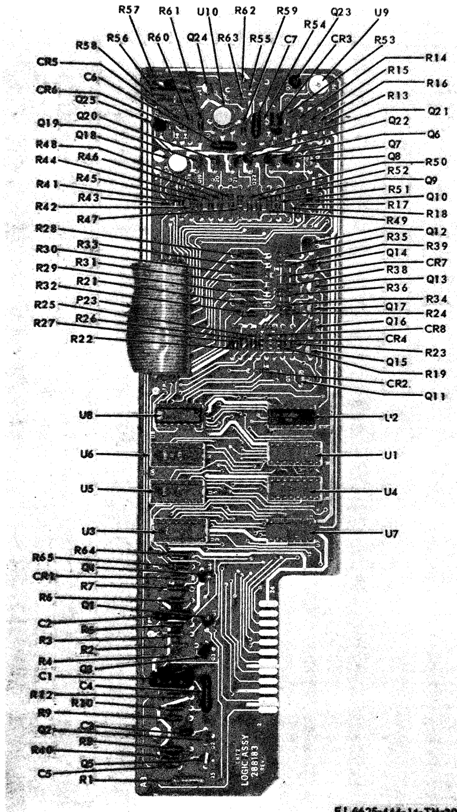
Figure 6-6. Logic (A8) component parts.
