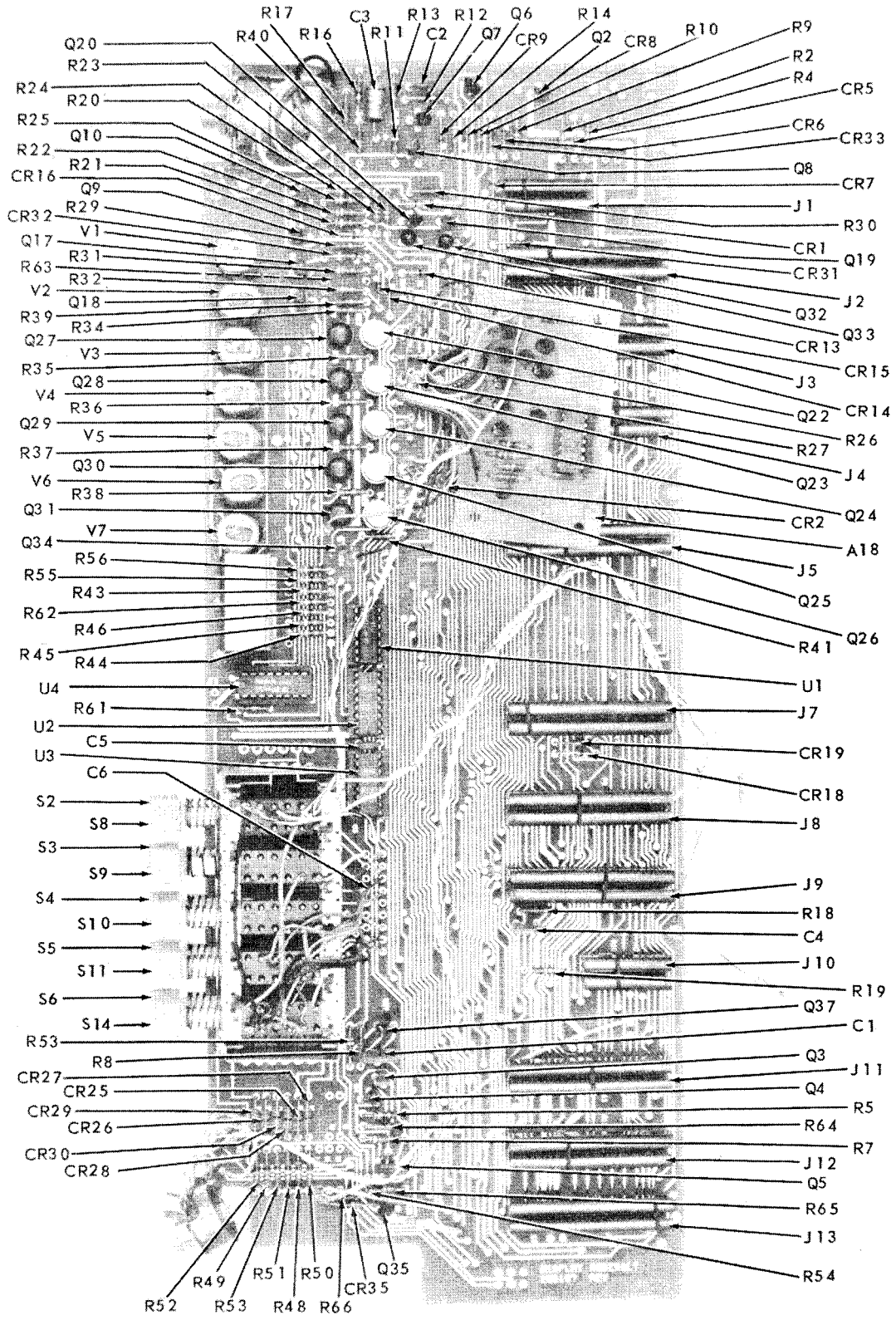
Figure 6-7. Display (A14) component parts.
