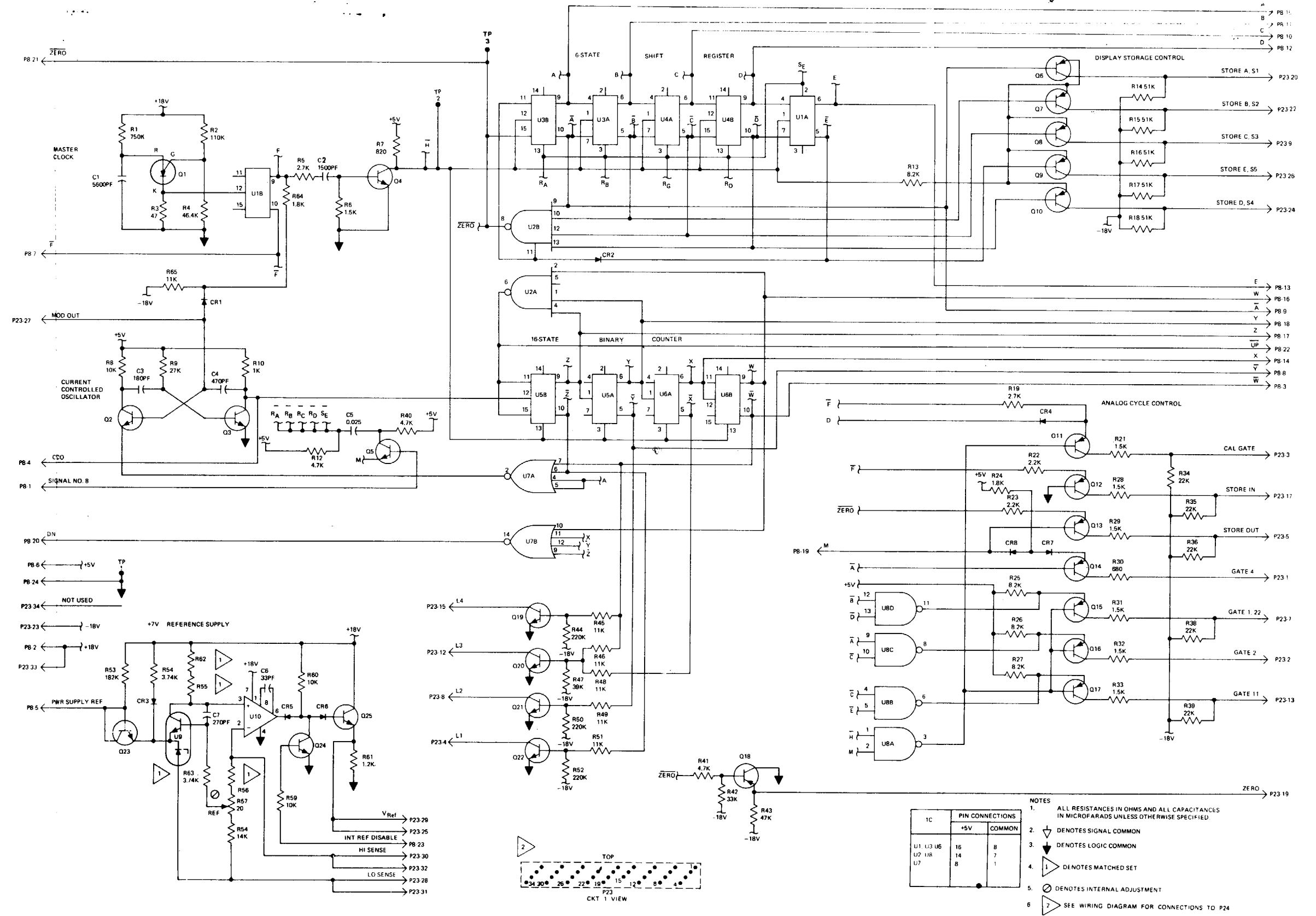
Figure FO-5. Logic (A8) schematic diagram.
