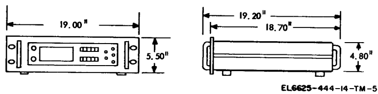
Figure 1-4. Outline drawing.
