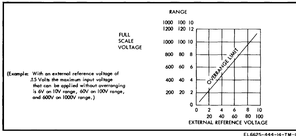
Figure 3-4. Ratio overrange limits.
