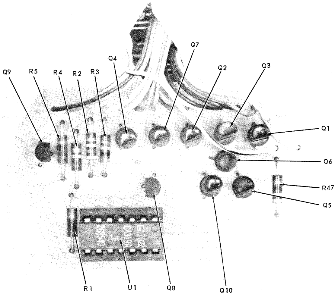
Figure 6-11. Decimal logic (A18) component parts.
