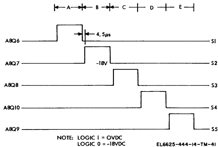
Figure 6-17. Analog storage waveforms.
